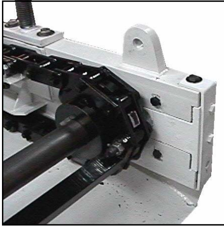
Slotted Siderails for Head and Tail Shaft removal
