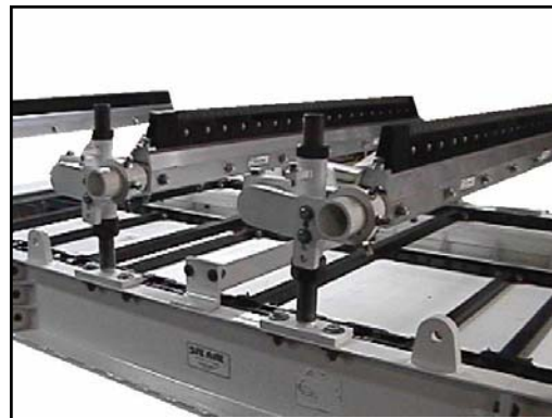
Belt Boss™ Mine Duty Cleaning Systems for effective cleaning on high speed mechanical spliced belts
