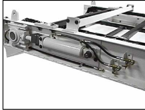
Grease Jack / Shim Set take-ups maintain proper chain tension and shaft alignment
